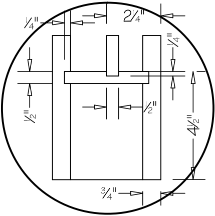
Track Section Detail Scale 1 \frac{1}{2}" = 1'-0"
