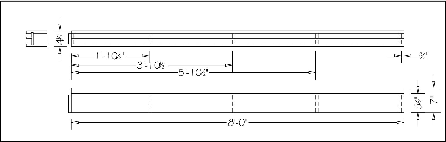
Track: Scale - \frac{3}{4}" = 1'-0" \frac{3}{4}" MDF construction with \frac{1}{2}" MDF sled shelf & divider
