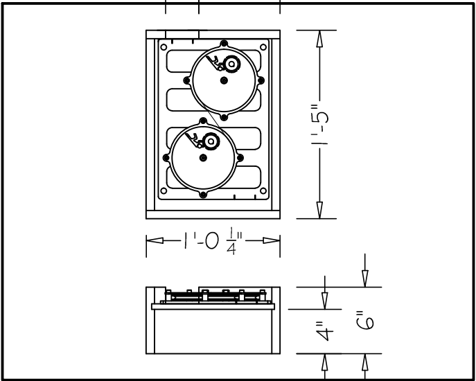
Turnaround block 1" = 1'-0" \frac{3}{4}" and \frac{1}{2}" MDF construction
